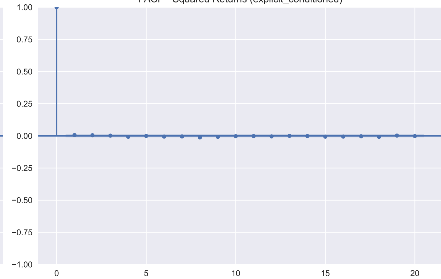
PACF - Squared Returns (explicit_conditioned)
