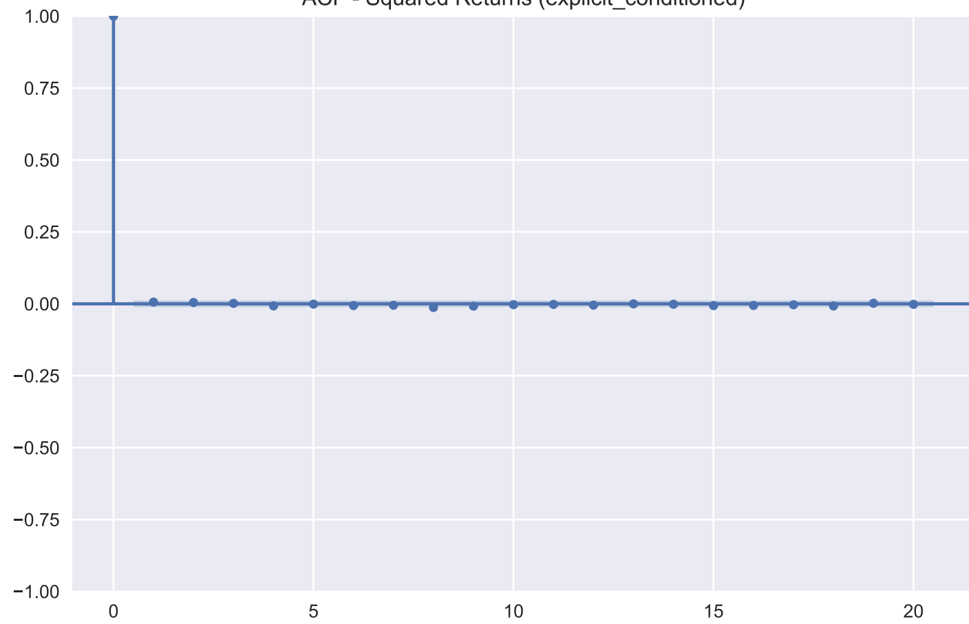
ACF - Squared Returns (explicit_conditioned)
